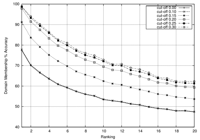
Figure 5. Protein Domain Membership Percentage Accuracy.
